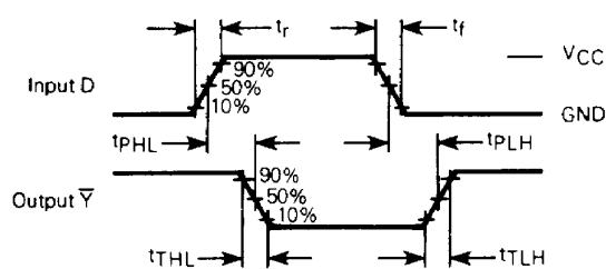
Figure 3. Switching Waveforms
