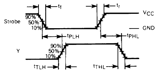
Figure 4. Switching Waveforms
